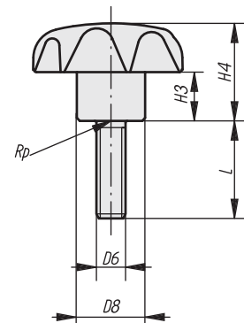
External thread version
