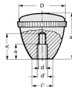
Plastic thread with counterbore
