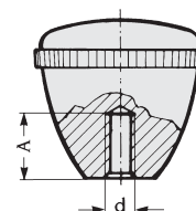
Plastic thread without counterbore
