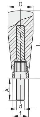
Male insert in zinc plated steel
