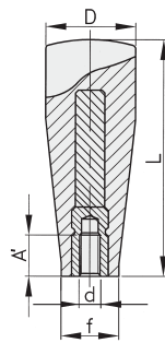
Female insert in zinc plated steel (except in brass for ref. 2557 and 2558)
