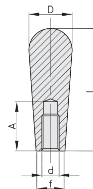
Plastic thread version
