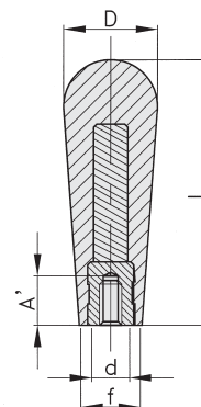
Zinc-plated steel insert
