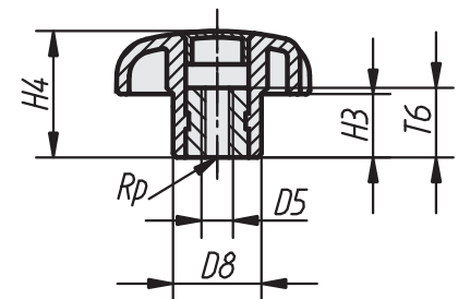
Internal thread version with protection cap
