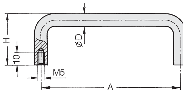
Handle supplied with M5x10 screws and washers
