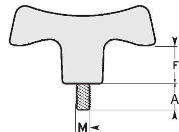
External thread version
