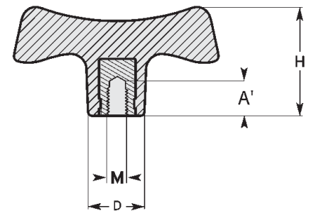
Internal thread version
