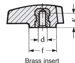
Brass insert
